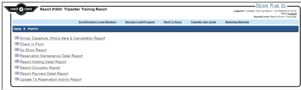
Figure 34 – Report Menu
