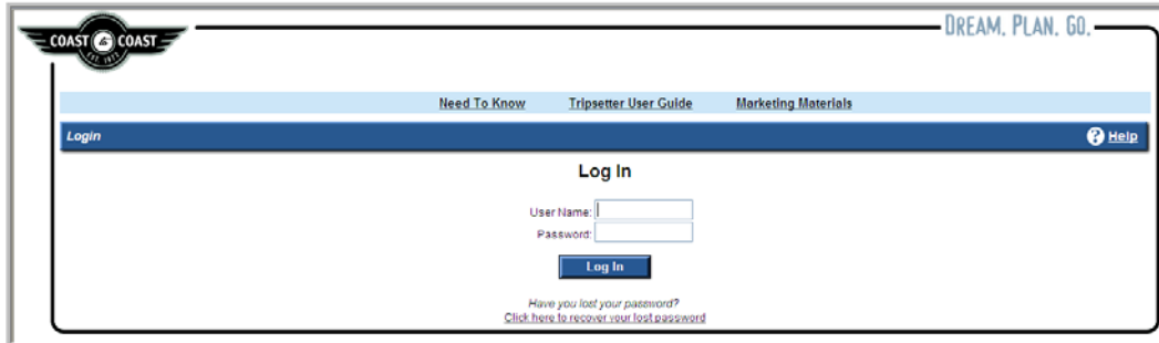
Figure 1 – Resort Login
